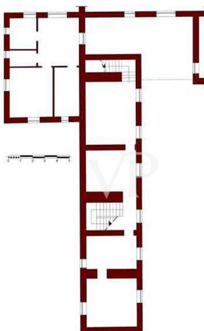
Piano Terra
